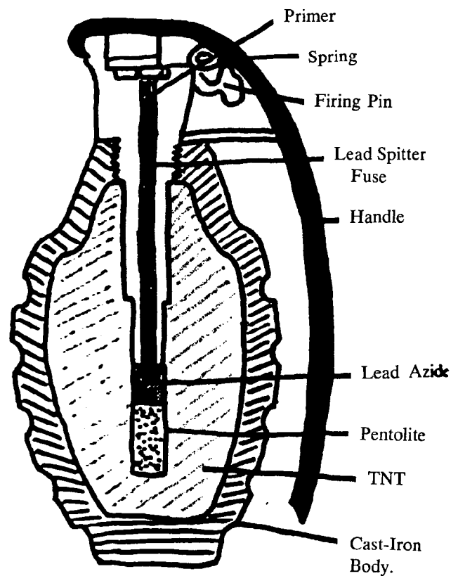
Figure 90. Military grenade.
