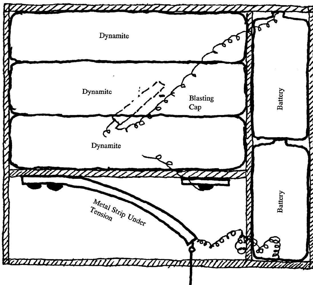
Figure 95. Tension-release detonator.
