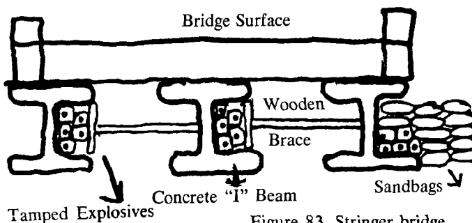
Figure 83. Stringer bridge.
