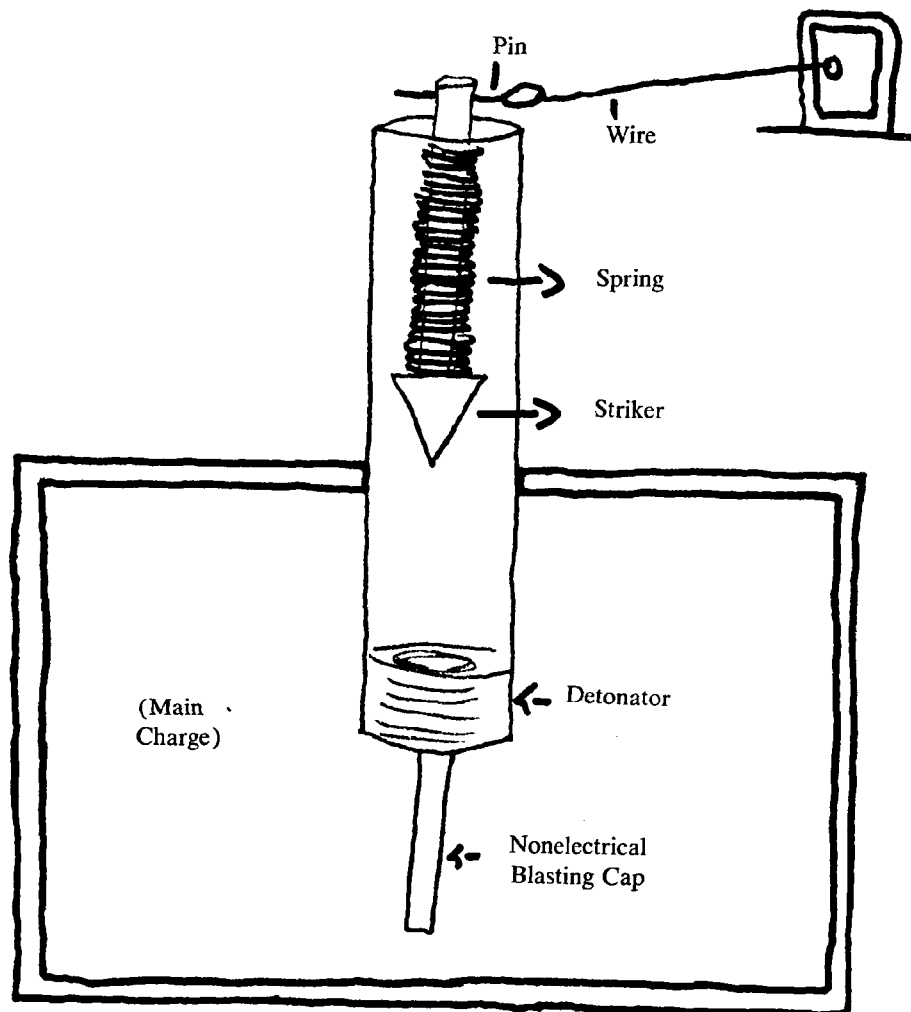
Figure 89. Tension-release detonator.
