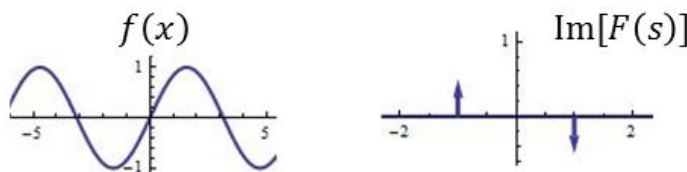
Figure 20.13: \sin(x) and its spectrum
