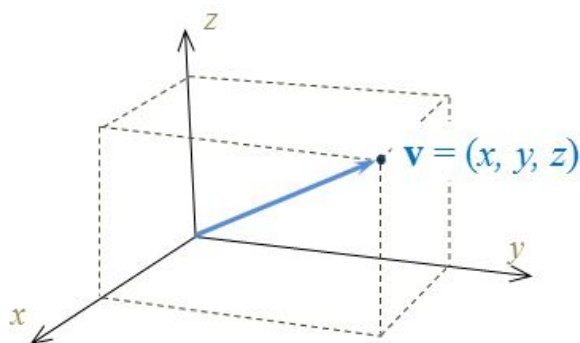
Figure 2.5: A vector in \mathbb{R}^3
