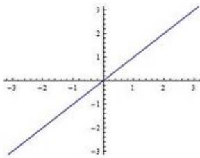
Figure 19.8: f(x) = x , when defined only on bounded domain [-\pi, \pi)
