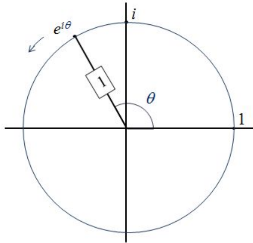
Figure 1.6: e^{i\theta} after \theta seconds, @ 2\pi rad/sec
