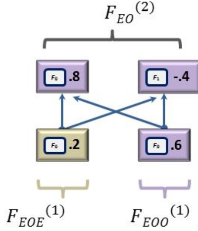
Figure 21.13: \left[F_{EO}^{(2)}\right]_j = \left[F_{EOE}^{(1)}\right]_{j \pmod{1}} + (-1)^{-j} \left[F_{EOO}^{(1)}\right]_{j \pmod{1}}
