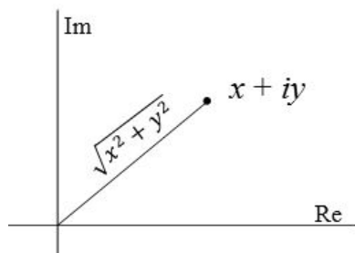
Figure 1.5: modulus of a complex number
