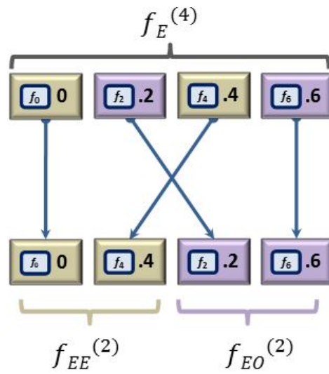
Figure 21.8: Decomposing the even 4-element array to two 2-element arrays (one even and one odd)
