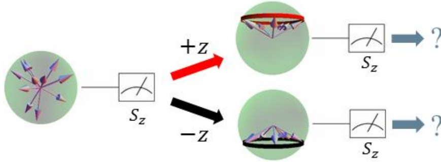
Figure 6.9: Plans for a follow-up to experiment # 1
