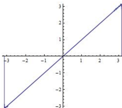
Figure 19.14: Fourier partial sum of f(x) = x to n = 1000
