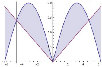
Figure 23.28: |\sin(x/2)| lies above |Kx/\pi| in the interval (-1.5\pi, 1.5\pi)
