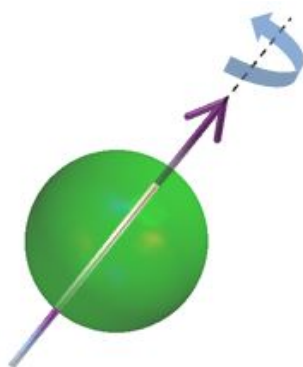
Figure 6.1: Classical angular momentum
