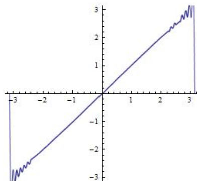
Figure 19.13: Fourier partial sum of f(x) = x to n = 50
