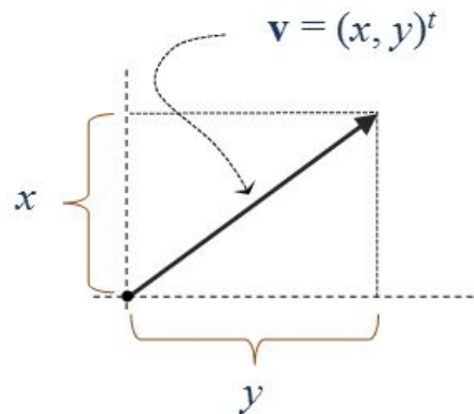
Figure 2.1: A vector in \mathbb{R}^2
