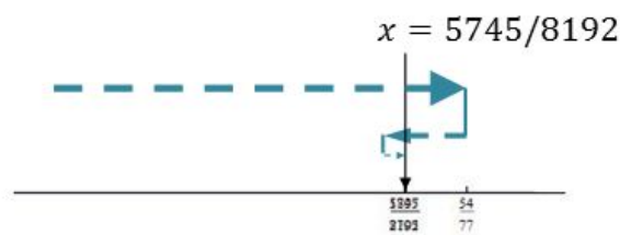
Figure 24.6: Fourth view of convergents
