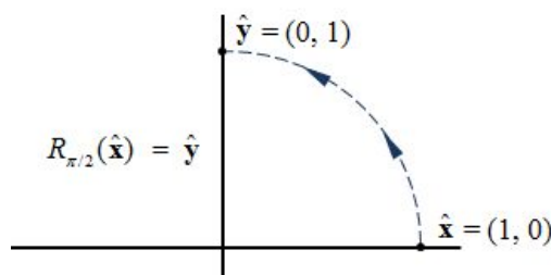
Figure 5.5: Rotation of \hat{\mathbf{x}} counter-clockwise by \pi/2
