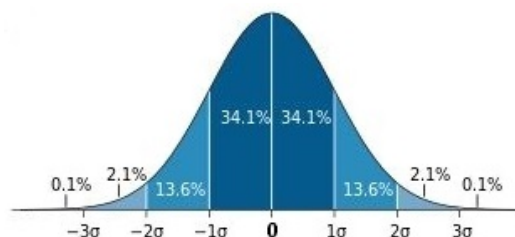
Figure 20.5: Interpretation of \sigma from Wikipedia Standard_deviation_diagram)
