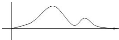
Figure 21.1: Continuous functions on a continuous domain
