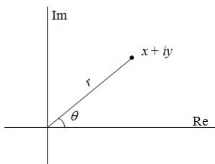
Figure 1.3: the connection between cartesian and polar coordinates of a complex number
