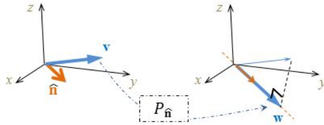
Figure 5.4: Projection onto an arbitrary direction \hat{\mathbf{n}}
