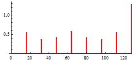
Figure 23.1: The spectrum of a vector with period 8 and frequency 16 = 128/8
