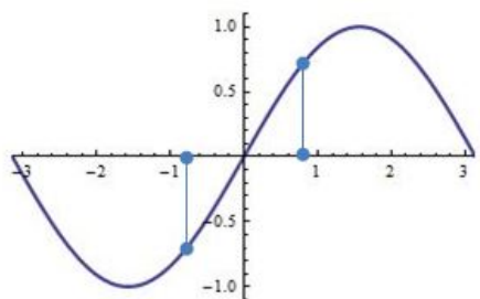
Figure 20.2: \sin x is odd
