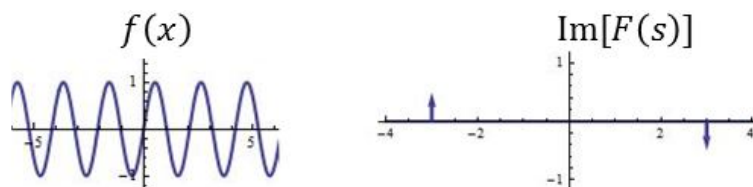
Figure 23.2: \sin(3x) and its spectrum
