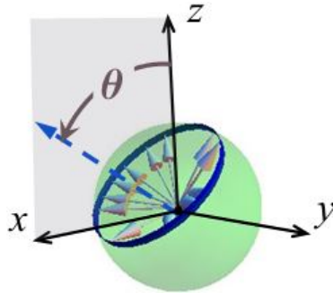
Figure 6.18: A spin direction with polar angle \theta from +z , represented by |\psi\rangle
