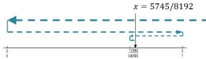
Figure 24.4: Second view of convergents
