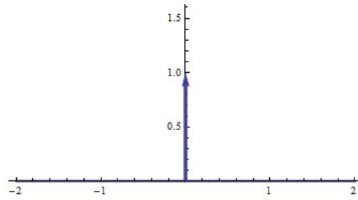
Figure 20.6: Graph of the Dirac delta function
