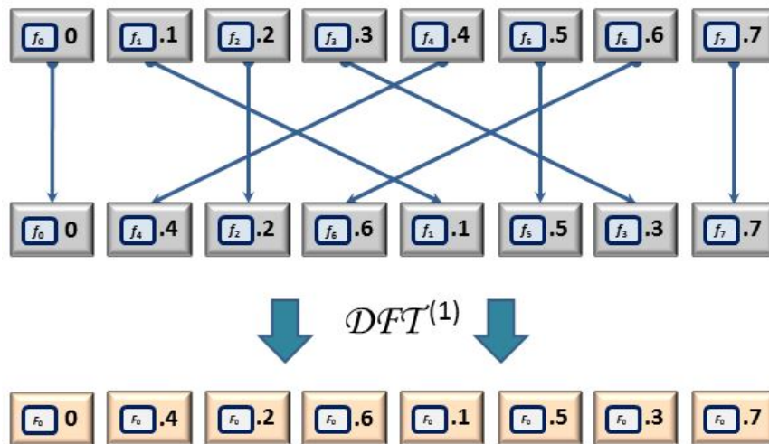
Figure 21.12: Bit-reversal reorders an eight-element array
