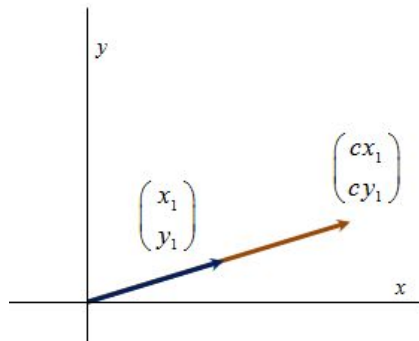
Figure 2.3: Scalar multiplication in \mathbb{R}^2
