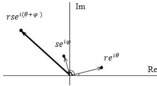
Figure 1.7: multiplication – moduli multiply and args add
