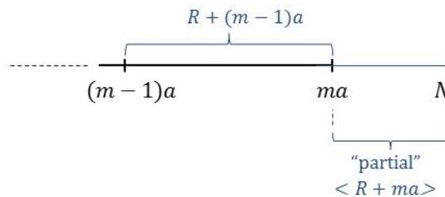
Figure 23.17: The final coset may have size < a
