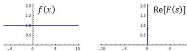
Figure 20.9: \mathcal{F}[1] is a 0-centered delta function
