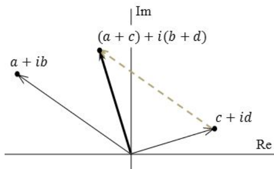
Figure 1.2: visualization of complex addition
