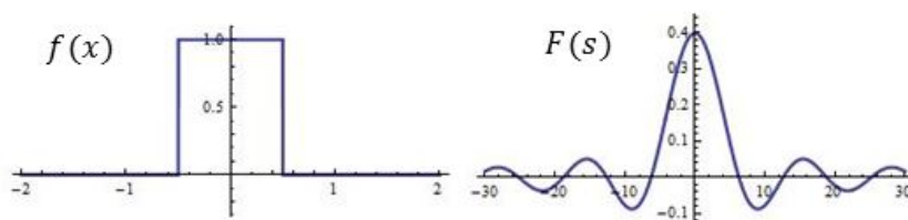
Figure 20.4: A simple function and its Fourier transform
