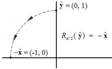
Figure 5.6: Rotation of \hat{\mathbf{y}} counter-clockwise by \pi/2
