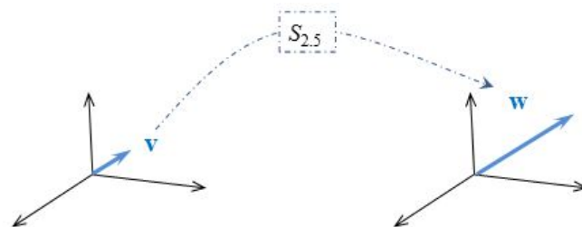
Figure 5.2: A scaling transformation
