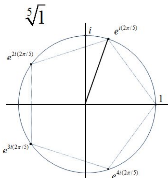
Figure 1.8: the fifth roots-of-unity
