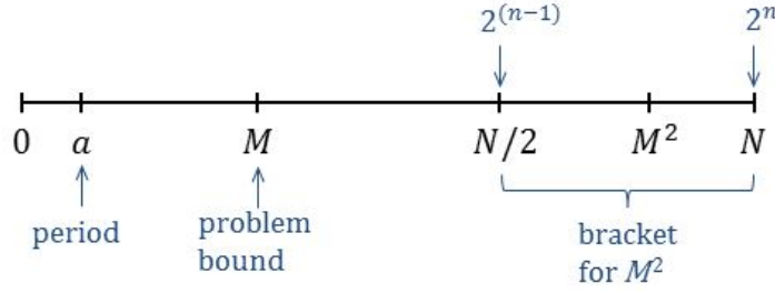
Figure 23.9: N = 2^n chosen so (N/2, N] bracket M^2
