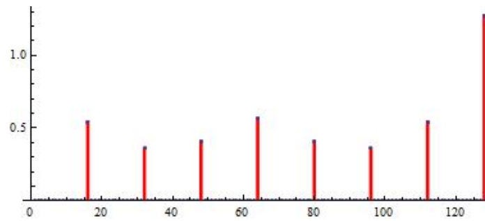
Figure 21.5: The spectrum of a periodic vector
