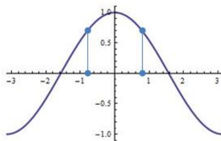
Figure 20.1: \cos x is even
