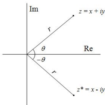
Figure 1.4: conjugation as reflection
