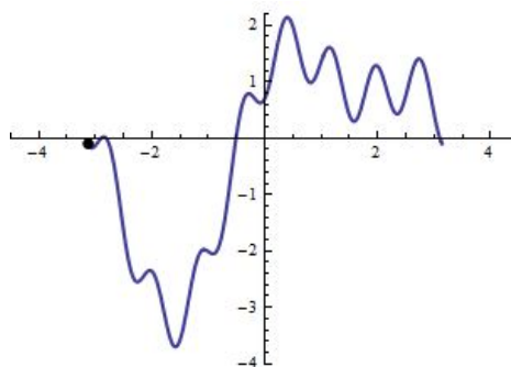
Figure 19.6: A function with bounded domain that can be expressed as a Fourier series
