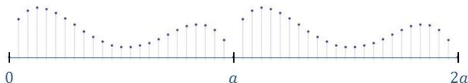
Figure 23.5: Example of a periodic function that is NOT periodic injective
