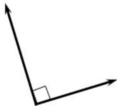
Figure 2.4: Orthogonal vectors
