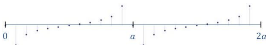
Figure 23.4: Graph of 2 periods of a periodic injective function
