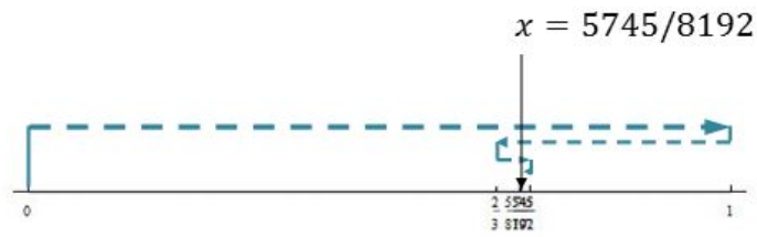
Figure 24.3: First view of convergents
