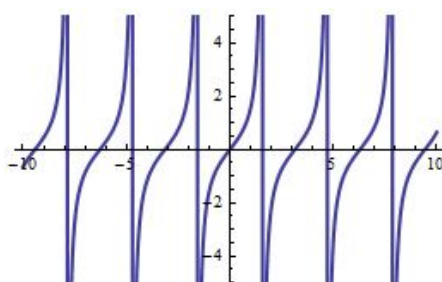
Figure 19.2: The function y = \tan x blows-up at isolated points but is still periodic (with period \pi )
