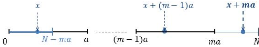
Figure 23.18: If 0 \leq x < N - ma , a full m + 1 numbers in \mathbb{Z}_N map to f(x)
