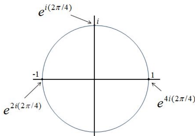
Figure 1.9: the fourth roots-of-unity
