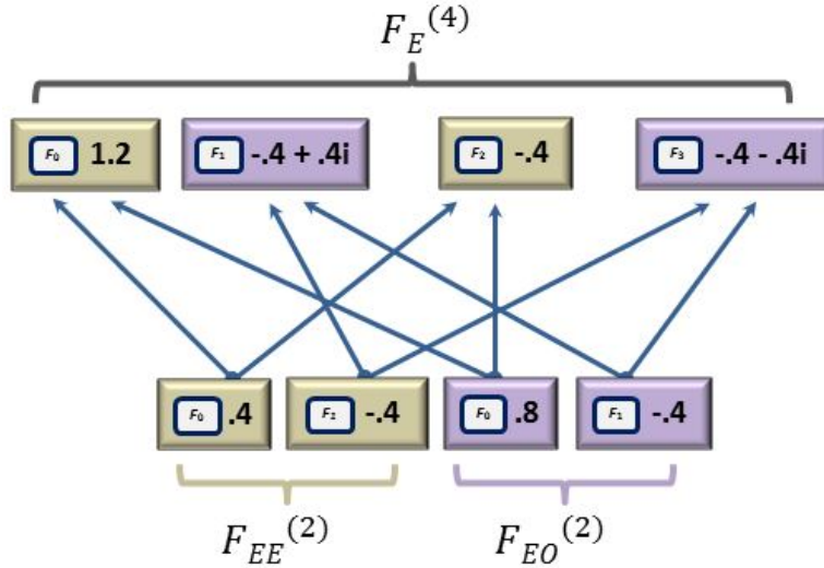
Figure 21.14: \left[F_E^{(4)}\right]_j = \left[F_{EE}^{(2)}\right]_{j \pmod{2}} + (i)^{-j} \left[F_{EO}^{(2)}\right]_{j \pmod{2}}
