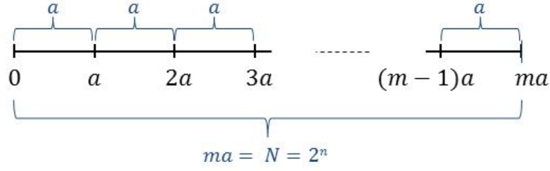
Figure 23.11: Easy case covers a \mid N , exactly
