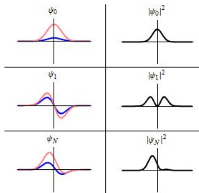
Figure 20.3: Square-integrable wavefunctions from Wikipedia StationaryStatesAnimation.gif
