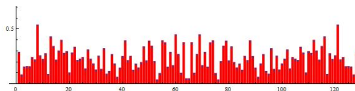
Figure 21.4: The \mathcal{DFT} of a non-periodic vector
