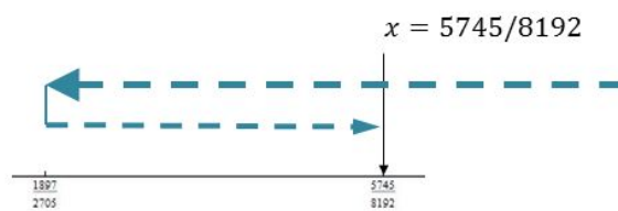
Figure 24.7: Fifth view of convergents
