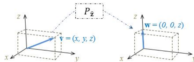
Figure 5.3: Projection onto the direction \hat{\mathbf{z}} , a.k.a. \hat{\mathbf{x}}_3
