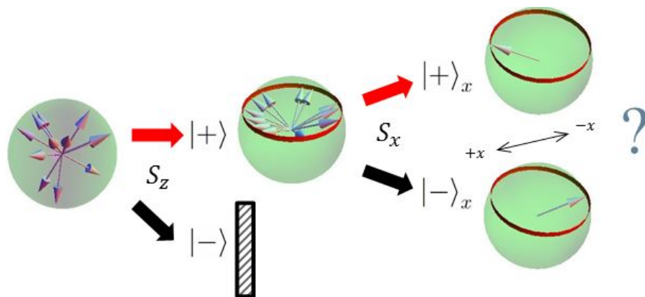
Figure 6.15: A guess about the states of two groups after experiment #2
