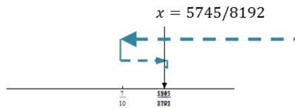
Figure 24.5: Third view of convergents
