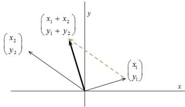
Figure 2.2: Vector addition in \mathbb{R}^2
