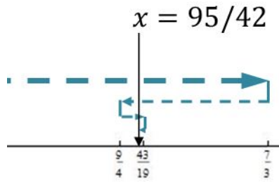
Figure 24.2: A close-up showing some of the latter convergents.
