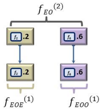
Figure 21.9: Breaking a two-element array into two singletons
