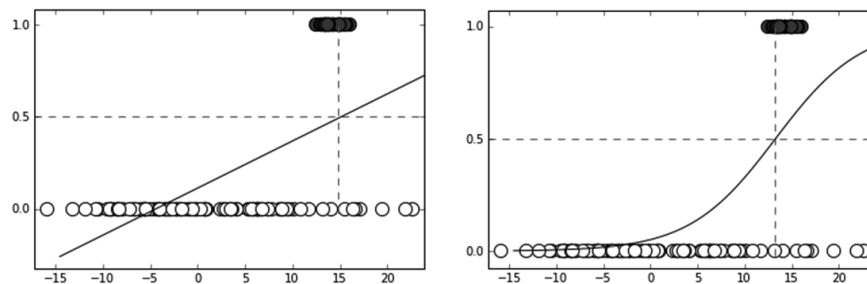
FIGURE 15-2: Probabilities do not work as well with a straight line as they do with a sigmoid curve.
