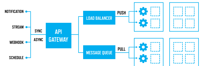
End-to-end lifecycle of a serverless workload
